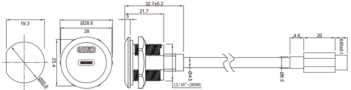
产品开孔尺寸 hole opening size
